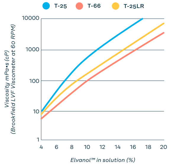
Figure 1: Effects of Concentration on Viscosity of Elvanol™ at 71 °C
